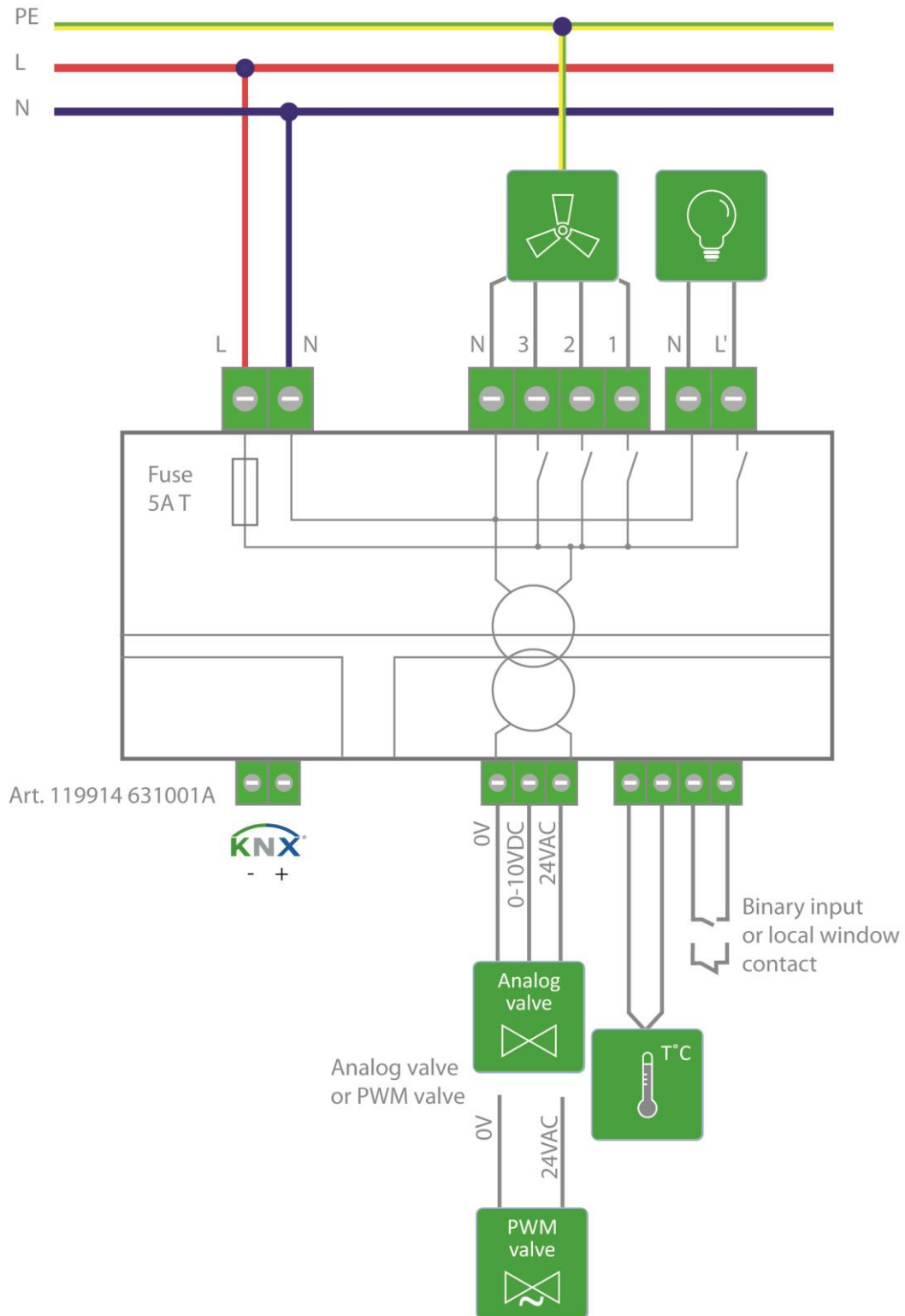
Figure 1: Connection diagram
