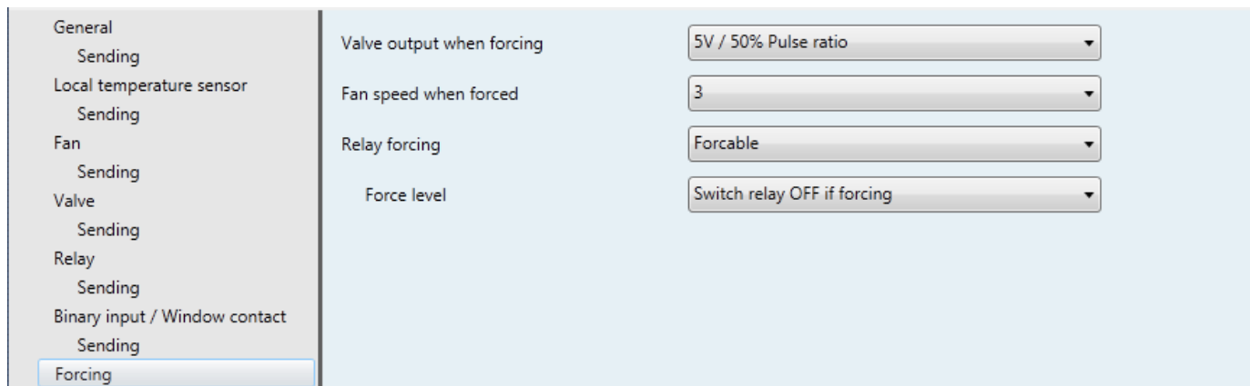
Figure 18: Forcing mode parameters
